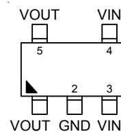
SOT-23-5 (L-Type)
